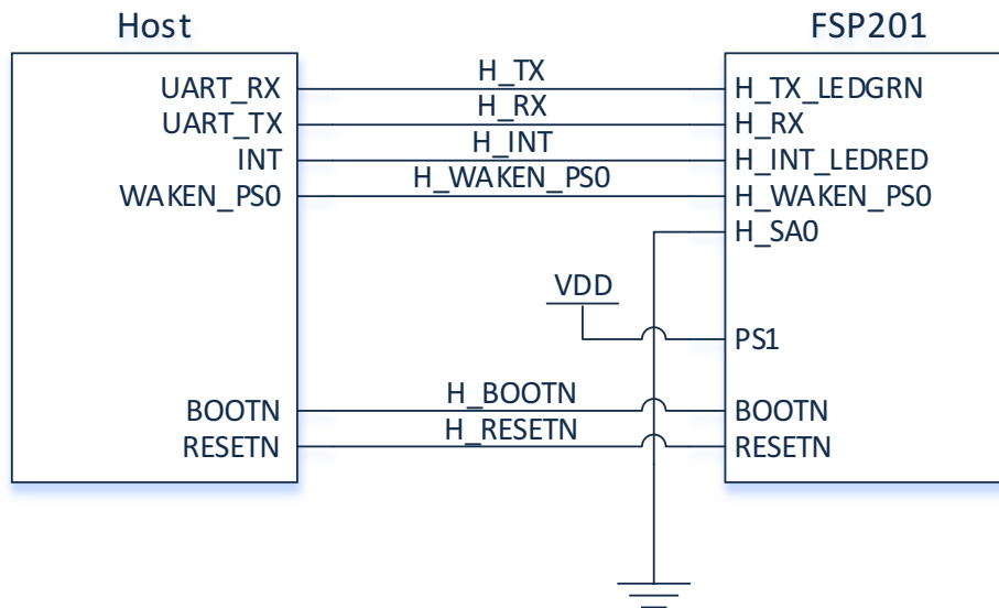
Figure 5: UART-SHTP Connection Diagram
