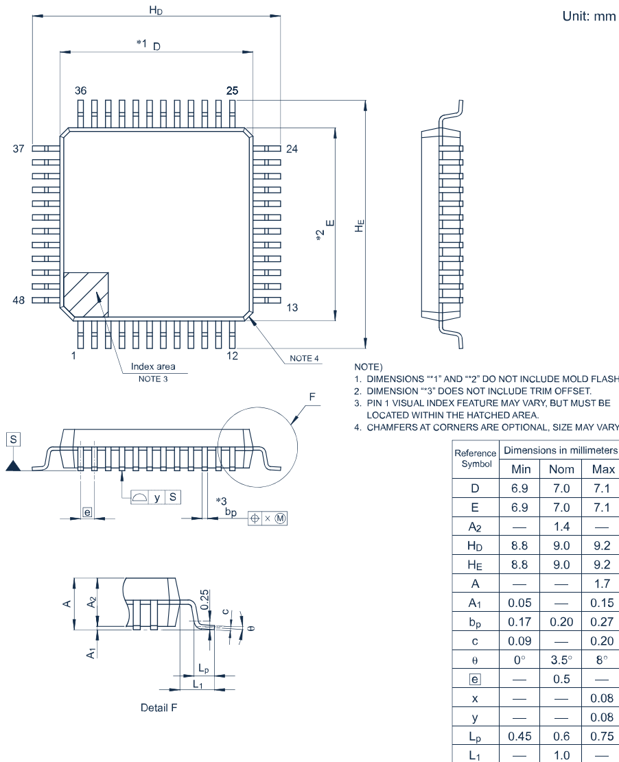
Figure 26 - LQFP48 Package
