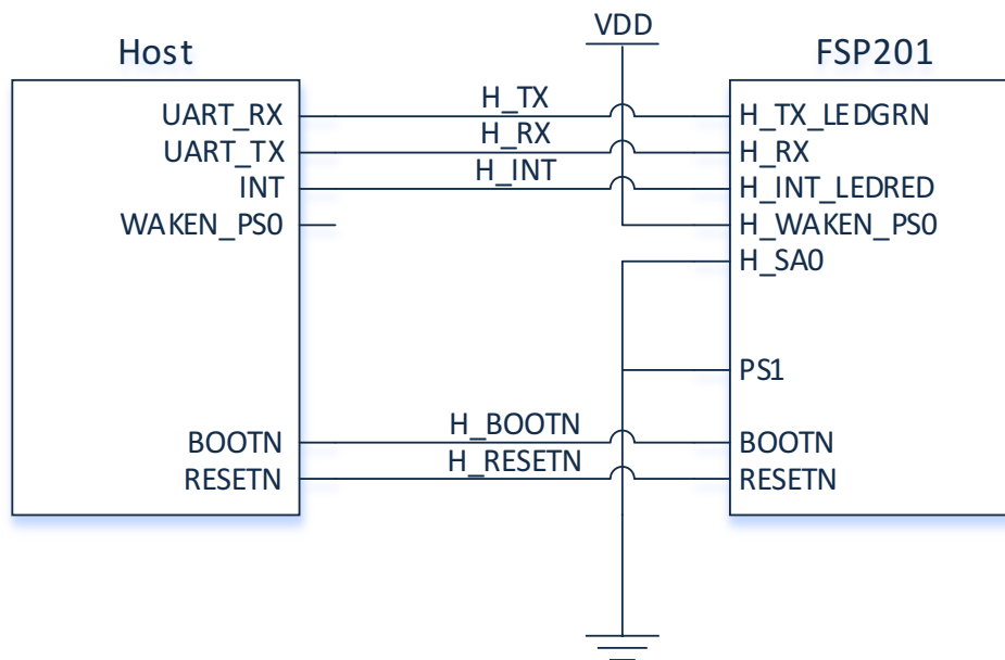
Figure 2: UART-RVC Connection Diagram
