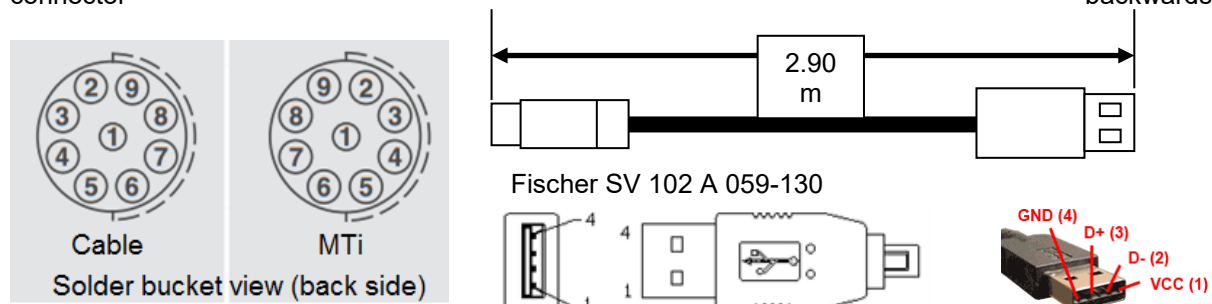
Figure 10: Drawing of CA-USB-MTi
